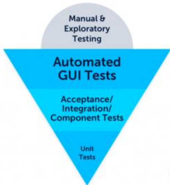
Automation "Ice Cream Cone" Anti-Pattern
